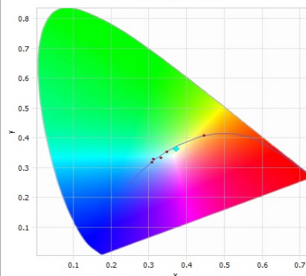
Chromatic Diagram(NW)
