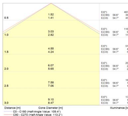
Conic Graph for Natural White Color
