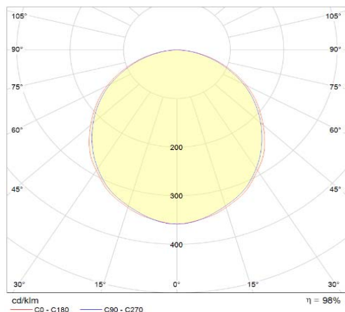
Polar Graph for Natural White Color
