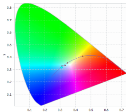
Chromaticity Diagram
