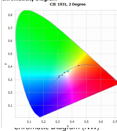
Chromaticity Diagram
