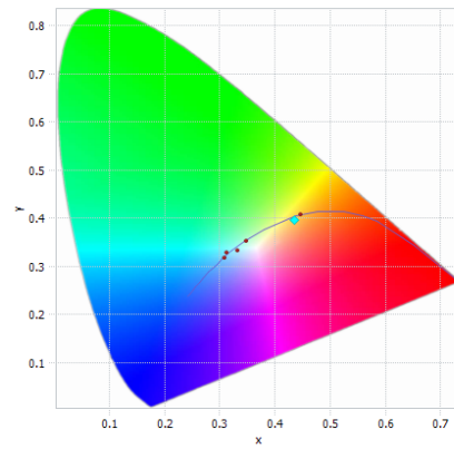
Chromaticity Diagram
